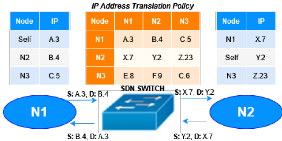
Figure 2.6: Example of SDN IP address translation adapted from Chiang, Venkatesan, et al. (2018)
