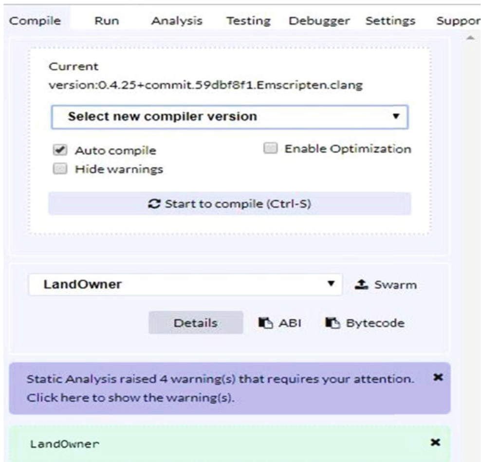
FIGURE 14: Compilation process.
