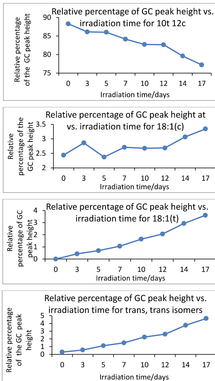
Figure 6: The graphs of relative percentage GC peak height vs. irradiation time for 18:1 (t), 18:1 (c), CLA 10t12c and CLA trans, trans isomers
