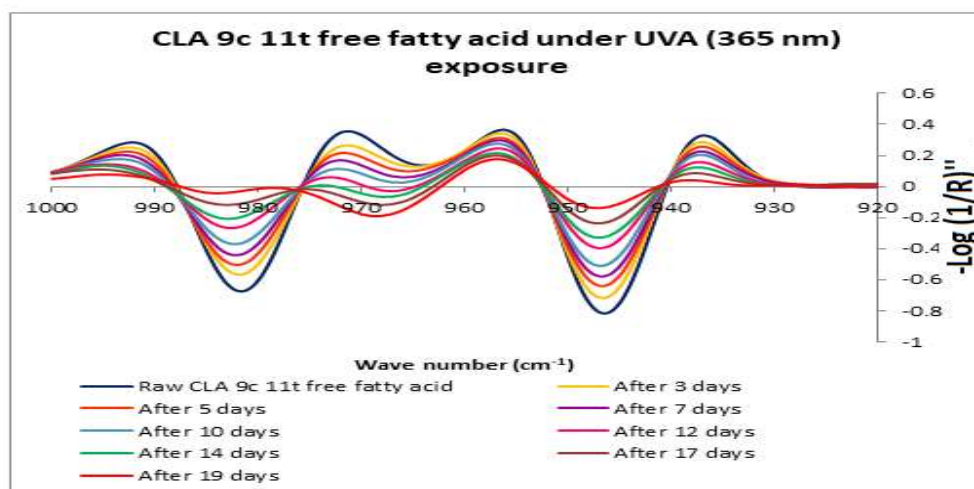
Figure 1: Second derivative profile of the infrared spectra of pure and UVA irradiated CLA 9c 11t free fatty acid in the region of 1000-920/cm
