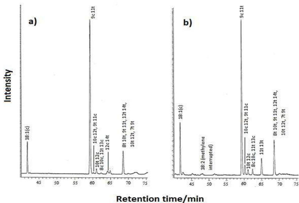
Figure 3: a) The gas chromatogram of FAME of the UVA irradiated CLA 9c 11t free fatty acid after 3 days b) The gas chromatogram of FAME of the UVA irradiated CLA 9c 11t free fatty acid after 19 days
