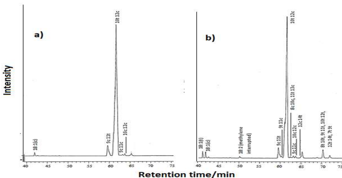
Figure 5: a) The gas chromatogram of raw 10t 12c-Octadecadienoic acid methyl ester b) 10t12c-Octadecadienoic acid methyl ester after 17 days
