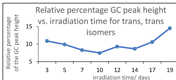
Figure 4: The graphs of relative percentage GC peak height vs. irradiation time for 18:1 (c), CLA 9c 11t and other trans, trans isomers
