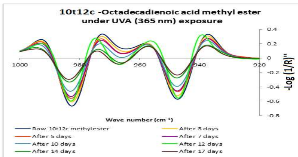
Figure 2: Second derivative profile of the infrared spectra of pure and UVA irradiated 10t12c-Octadecadienoic acid methyl ester in the region of 1000-920/cm
