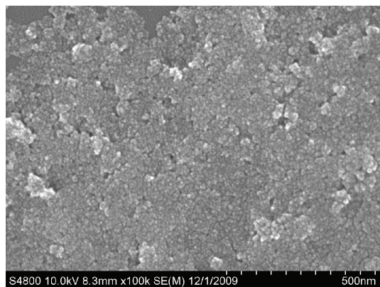
FIGURE 3: SEM micrograph of as-synthesized 10 mol% \text{La}_2\text{O}_3 doped \text{CeO}_2 .
