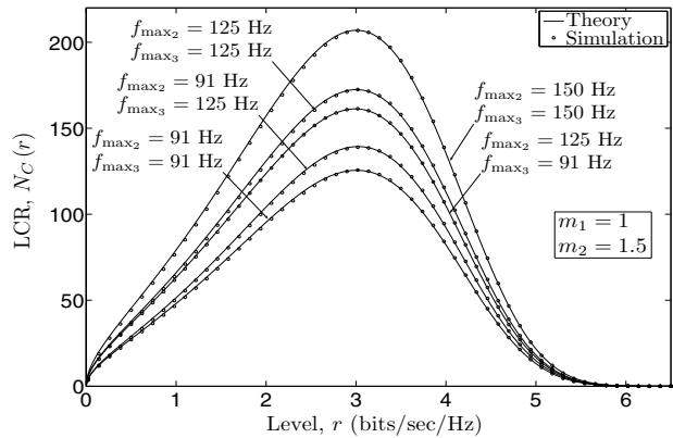
Fig. 7. The LCR N_C(r) of the capacity of double Nakagami- m channels.
