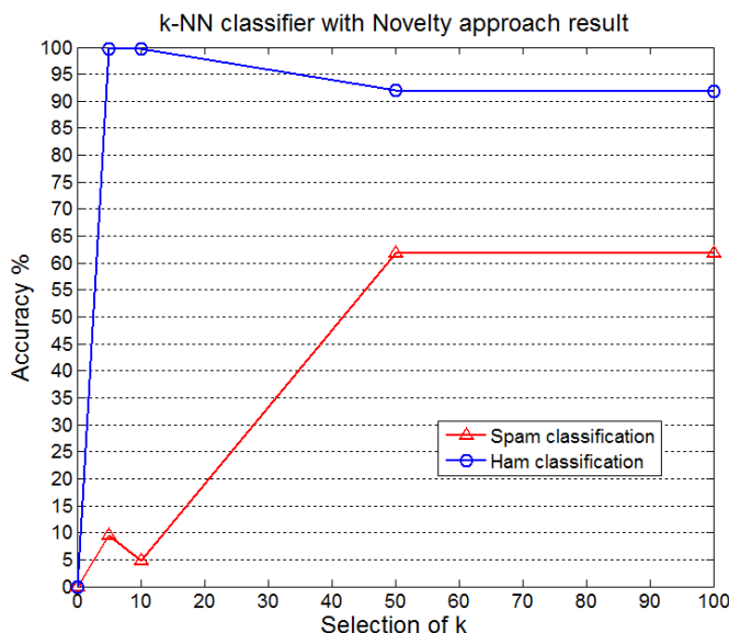
Figure 5-5 k-NN with Novelty detection experiment
