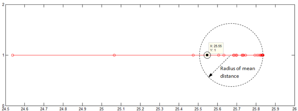
Figure 5-2 Naïve Bayes with Novelty detection experiment 2
