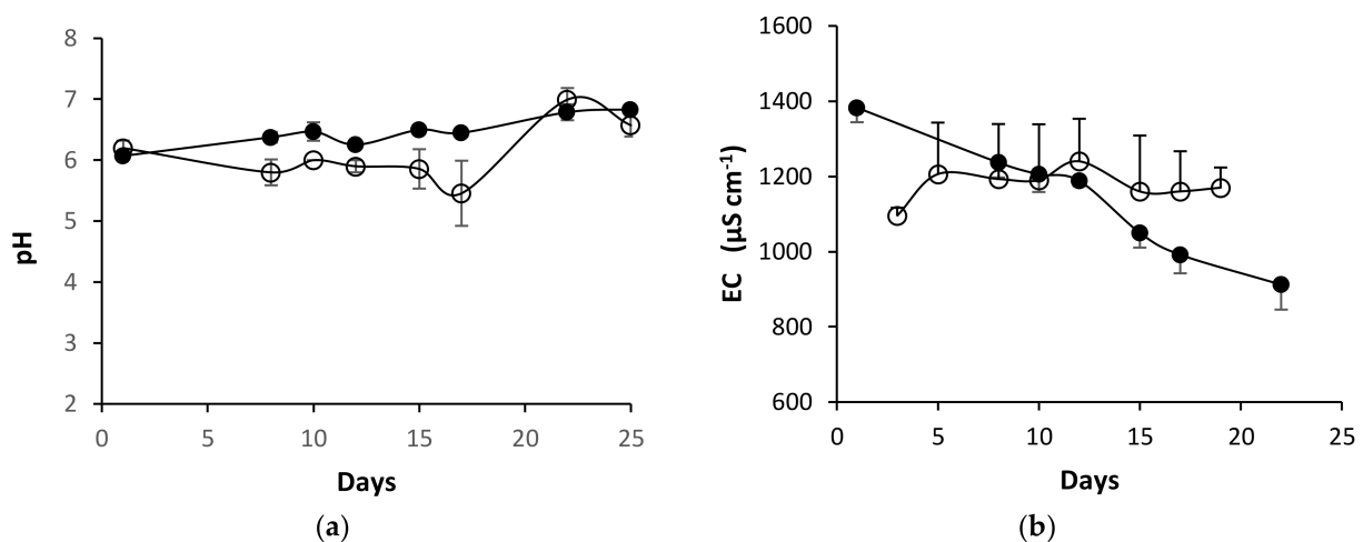
Figure 2. Variation in (a) pH and (b) EC in the organic (●) and conventional (○) nutrient solution over the 25 days experimental period.
