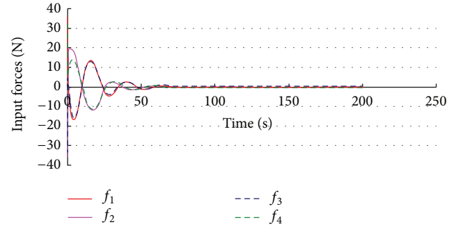
FIGURE 10: Input forces.
