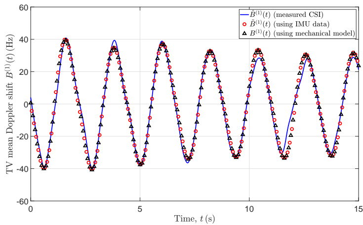
Figure 6. TV mean Doppler shifts \hat{B}^{(1)}(t) , B^{(1)}(t) , and B^{(1)}(t) computed from the spectrograms of the channel model with IMU data as inputs, mechanical model as inputs, and the measured CSI, respectively.
