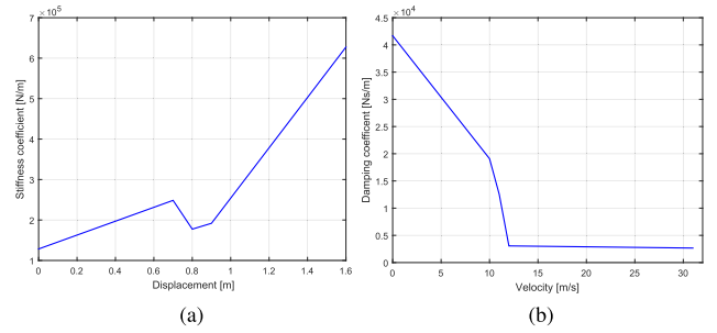
FIGURE 10. Piecewise spring and damper coefficients of the Caravan's front structure. (a) Stiffness coefficients. (b) Damping coefficients.
