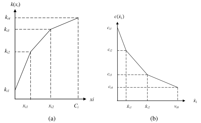
FIGURE 5. Predefined stiffness and damping coefficient characteristics of the vehicle's front structure. (a) Stiffness coefficients. (b) Damping coefficients.
