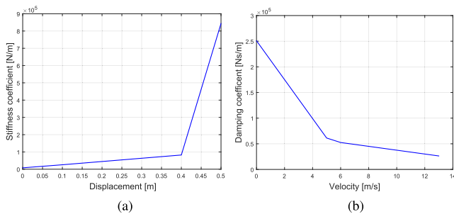
FIGURE 13. Piecewise spring and damper coefficients of the Chevrolet's front structure. (a) Stiffness coefficients. (b) Damping coefficients.
