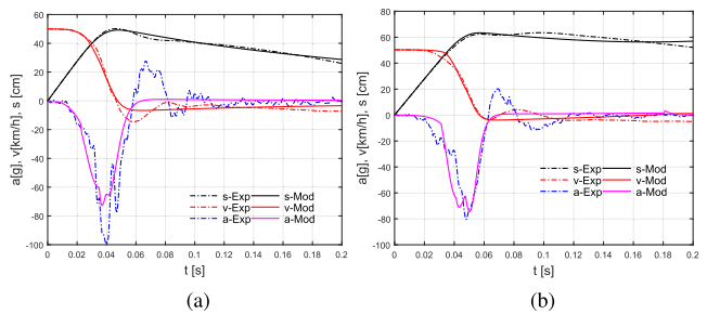
FIGURE 11. Model vs Experimental results for Dodge-to-Chevrolet crash using GA. (a) Dodge. (b) Chevrolet.
