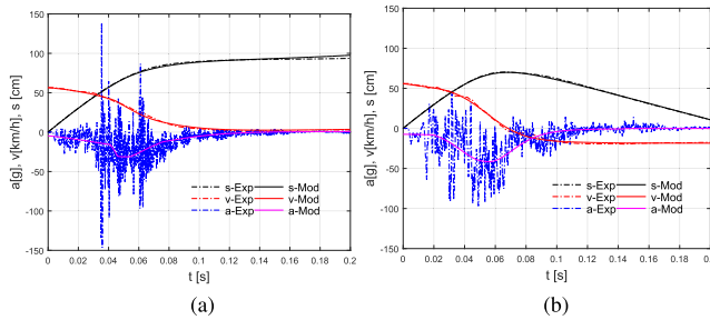
FIGURE 8. Model vs Experimental results for vehicle-to-vehicle (Caravan-Neon) crash using GA. (a) Caravane. (b) Neon.
