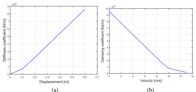
FIGURE 12. Piecewise spring and damper coefficients of the Dodge's front structure. (a) Stiffness coefficients. (b) Damping coefficients.
