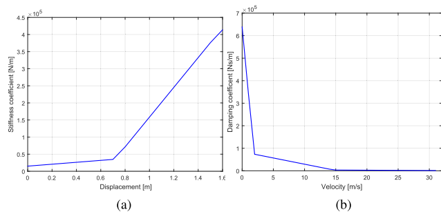
FIGURE 9. Piecewise spring and damper coefficients of the Neon's front structure. (a) Stiffness coefficients. (b) Damping coefficients.
