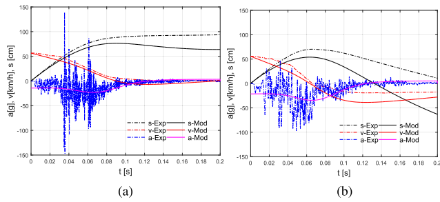
FIGURE 7. Model vs Experimental results for vehicle-to-vehicle (Caravan-Neon) crash using IPA. (a) Caravan. (b) Neon.
