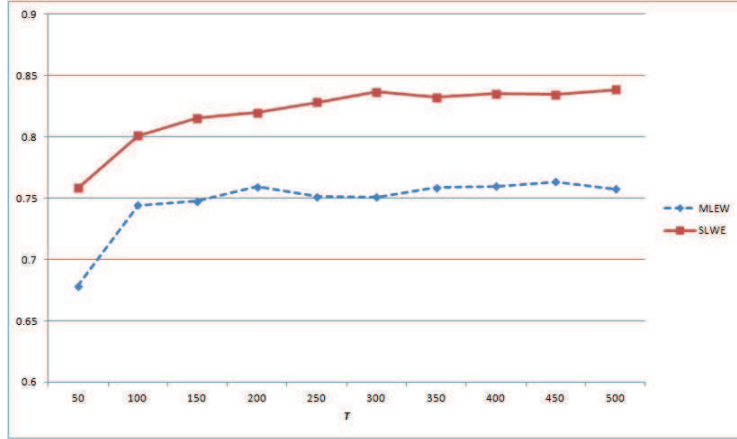
Figure 9: Plot of the accuracies of the MLEW and the SLWE multinomial classifiers on a one-dimensional dataset generated from two non-stationary sources with different switching periods, as described in Table 6.
