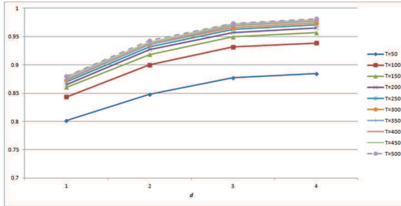
Figure 13: Plot of the accuracies of the SLWE classifier for different multinomial( r=4 ) datasets with different dimensions, d , over different values of the switching periodicity, T . The numerical results of the experiments are shown in Table 10.
