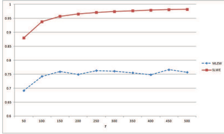
Figure 11: Plot of the accuracies of the MLEW and the SLWE multinomial classifiers on a 3-dimensional dataset generated from two non-stationary sources with different switching periods, as described in Table 8.
