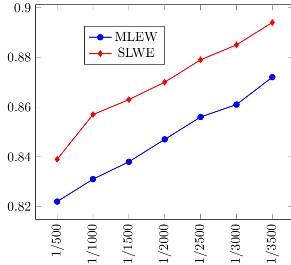
Figure 17: The ensemble results obtained for 50 simulations with the dimension of the data 30 corresponding to Table 11.
