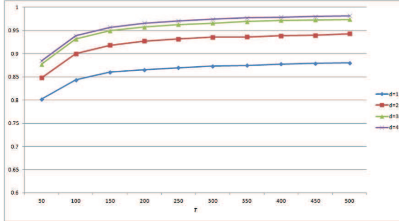
Figure 13: Plot of the accuracies of the SLWE classifier for different multinomial( r=4 ) datasets with different dimensions, d , over different values of the switching periodicity, T . The numerical results of the experiments are shown in Table 10.
