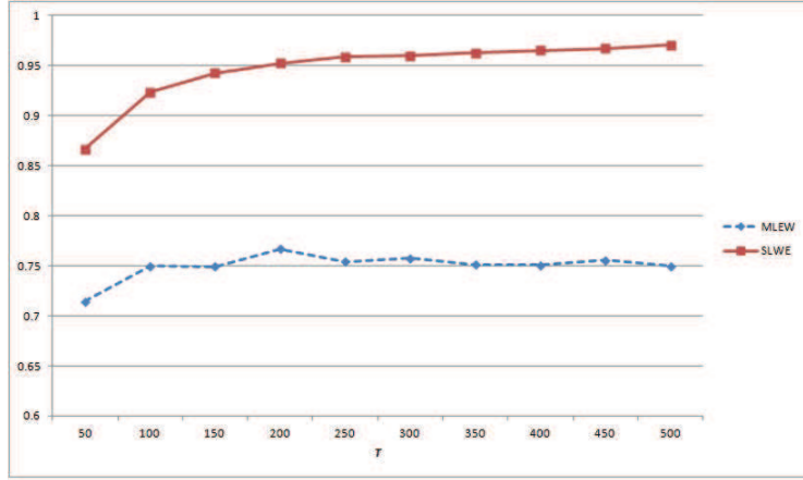
Figure 6: Plot of the accuracies of the MLEW and the SLWE binomial classifiers on a 4-dimensional dataset generated from two non-stationary sources with different switching periods, as described in Table 4.
