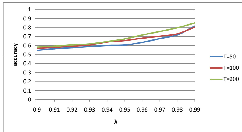
Figure 16: Plot of the classification accuracy of the SLWE classifier for different values of T and the update parameter, \lambda , for the real-life application.
