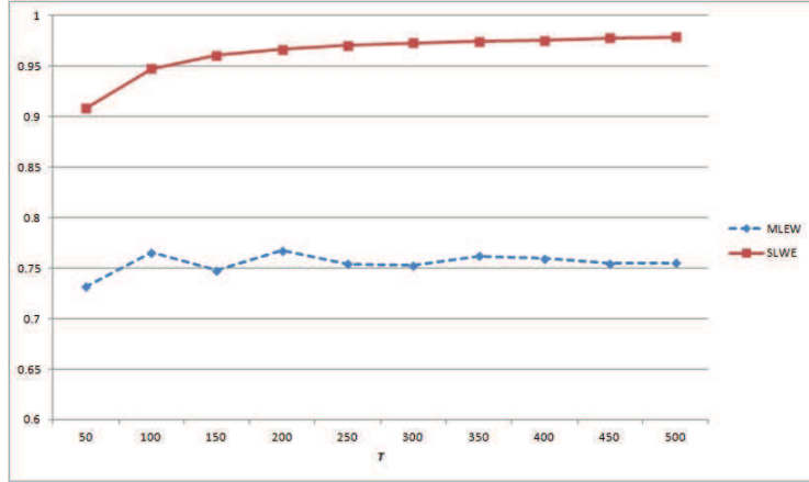
Figure 4: Plot of the accuracies of the MLEW and the SLWE binomial classifiers on a 2-dimensional dataset generated from two non-stationary sources with different switching periods, as described in Table 2.
