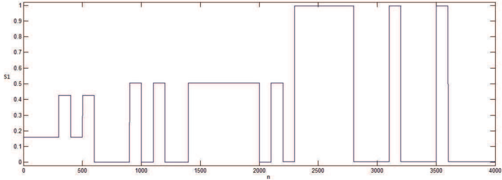
Figure 2: An example of the true underlying probability of ‘0’, S_1 , for a one-dimensional binary data stream. The data was generated using two different sources in which the period of switching was 100, and the stochastic properties of the classes switched two times.
