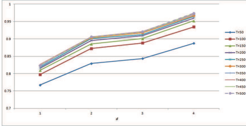
Figure 8: Plot of the accuracies of the SLWE classifier for different binomial datasets involved data from two non-stationary classes. Each dataset was generated with a different switching period, T , and a different dimensionality, d . The numerical results of the experiments are shown in Table 5.
