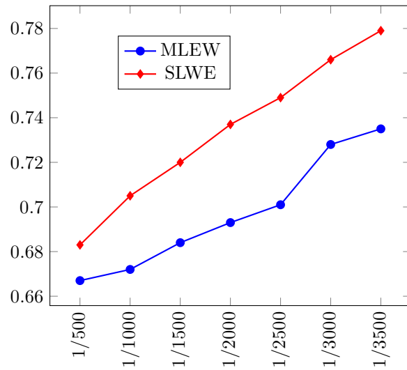
Figure 18: The ensemble results obtained for 50 simulations with the dimension of the data 10 corresponding to Table 12.
