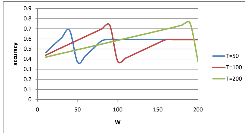
Figure 15: Plot of the classification accuracy of of the MLEW classifier for different values of T and size of the window, W , for the real-life application.
