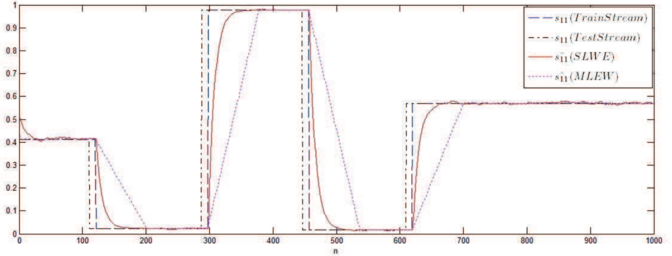
Figure 1: Plot of the averages for the estimates of s_{11} , obtained from the SLWE and MLEW at time n , using the available training samples that arrived with the delay of t_d = 10 . The stochastic properties of each class switched four times at randomly selected times.
