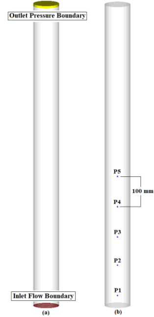
Figure 2. (a) Boundary conditions, (b) Pressure points Five different meshes with 6656, 9000, 16819, 22176 and 27378 cells were tested and cross sectional views are illustrated in Figure 3.
