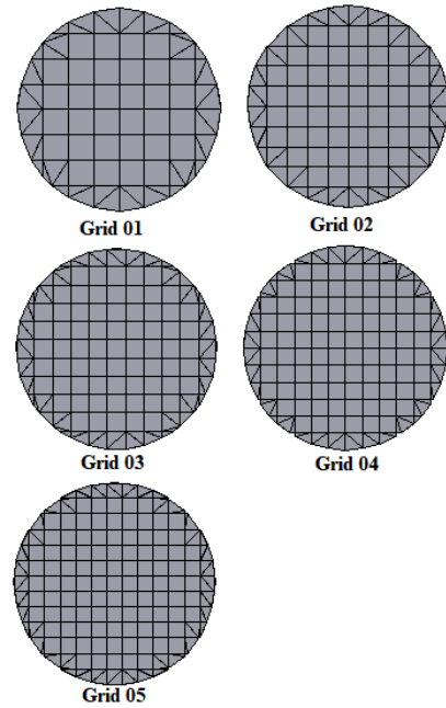
Figure 3. Cross sectional views of different grids
