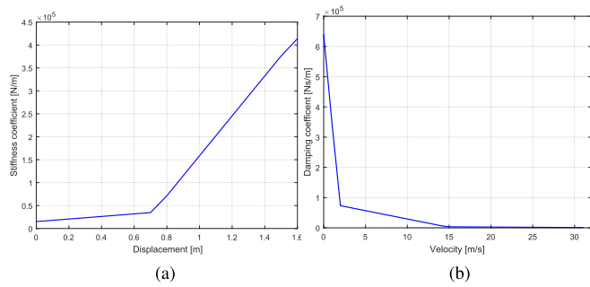
FIGURE 9. Piecewise spring and damper coefficients of the Neon's front structure. (a) Stiffness coefficients. (b) Damping coefficients.
