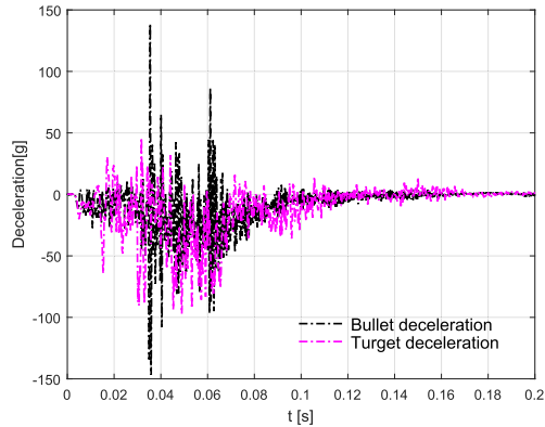
FIGURE 2. Test decelerations for bullet and target vehicles.
