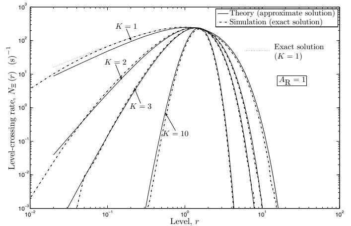
Fig. 4. The LCR N_{\Xi}(r) of the received signal envelope at the output of the EG combiner \Xi(t) for a different number of diversity branches K .
