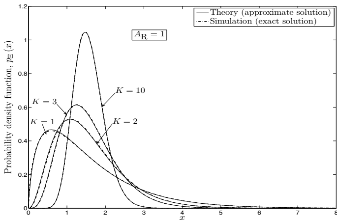
Fig. 2. The PDF p_{\Xi}(x) of the received signal envelope at the output of the EG combiner \Xi(t) for a different number of diversity branches K .
