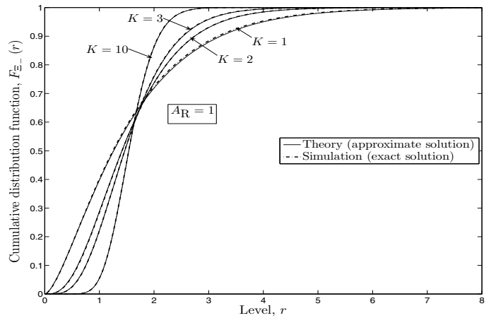
Fig. 3. The CDF F_{\Xi}(r) of the received signal envelope at the output of the EG combiner \Xi(t) for a different number of diversity branches K .
