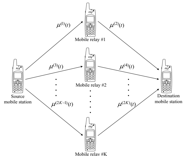
Fig. 1. The propagation scenario describing K -parallel dual-hop relay M2M fading channels.
