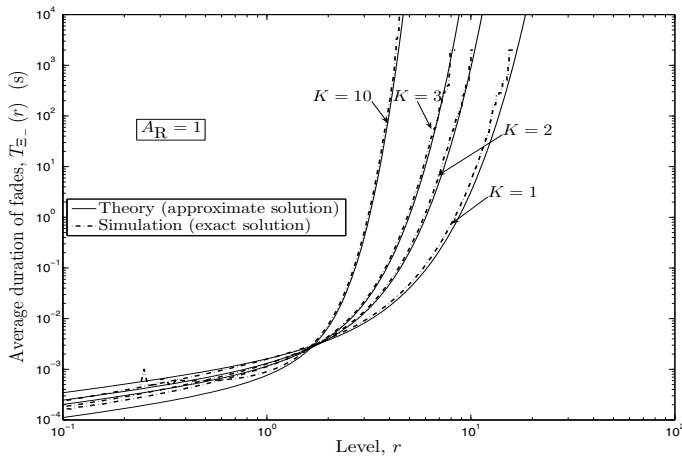
Fig. 5. The ADF T_{\Xi}(r) of the received signal envelope at the output of the EG combiner \Xi(t) for a different number of diversity branches K .
