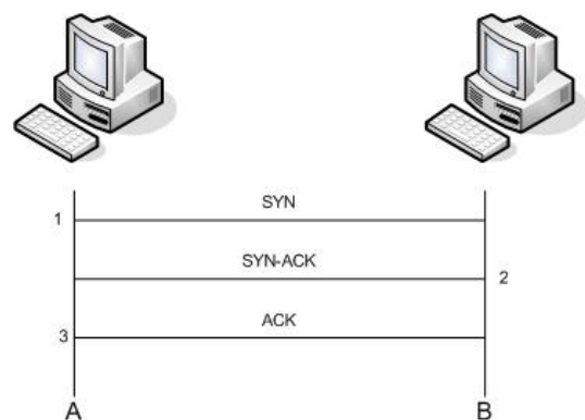
Figure 5 : Three-Way-Handshake
