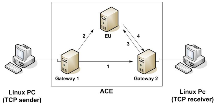
Figure 12 : Emulation of the Characteristic Model
