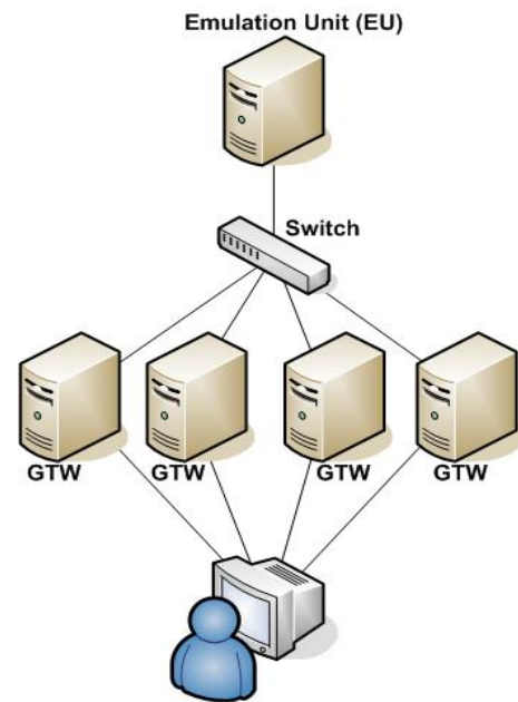
Figure 8 : Emulator Architecture
