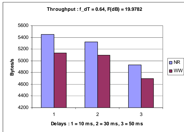
Graph 28 : Throughput : f_{dT} = 0.64 , F(\text{dB}) = 19.9782
