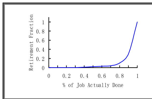
Figure 40: Retirement Function
