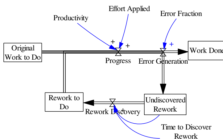
Figure 1: Rework Cycle
