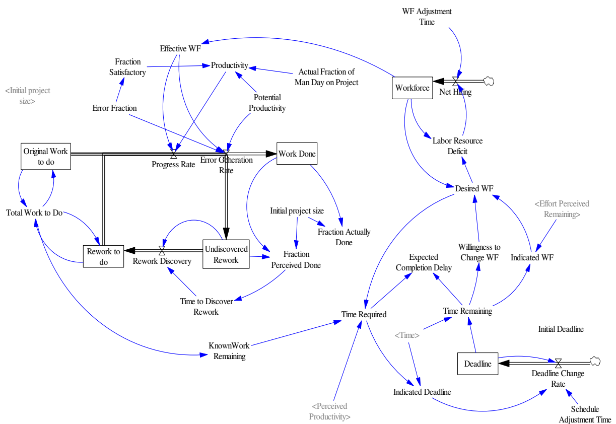
Figure 6: Basic model
