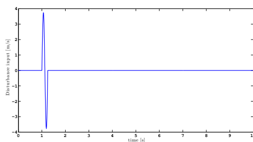
Fig. 6. Bump-like disturbance input.
