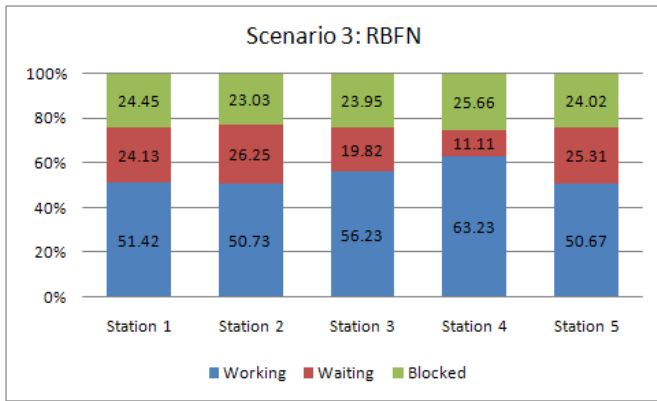
Fig. 11. Processing Times with RBFN in scenario 3.
