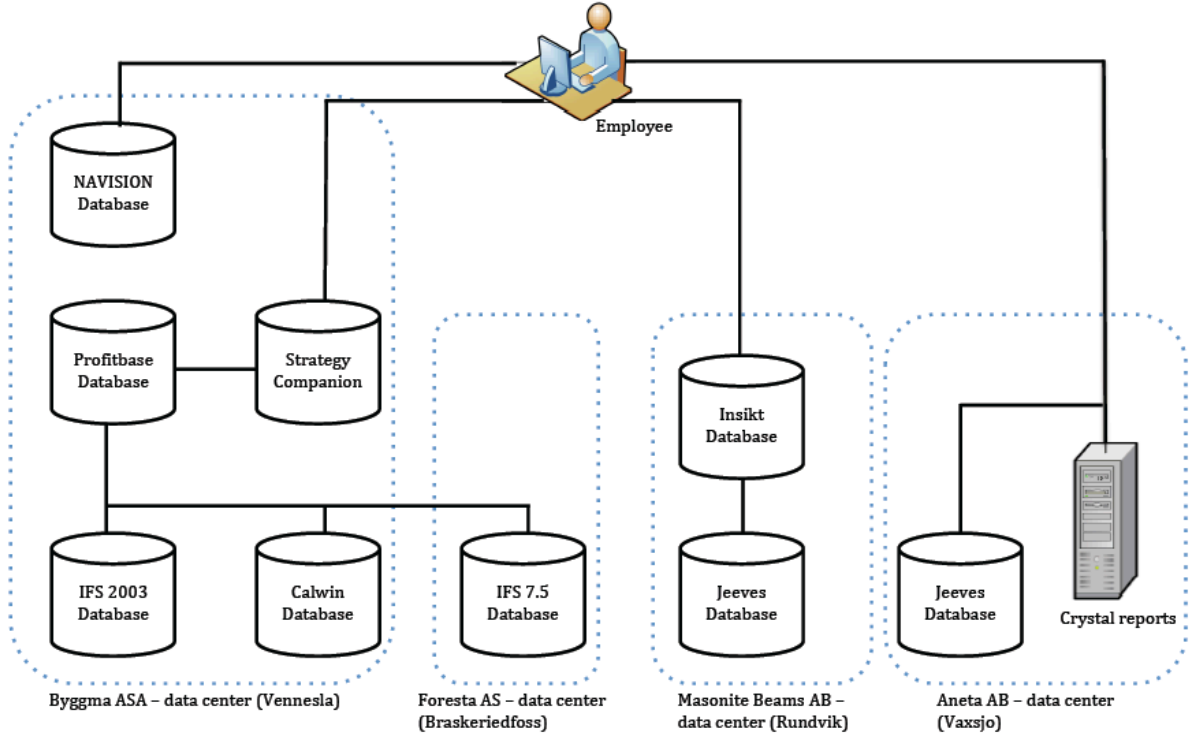
Figure 15 - Byggma ASA IT architecture
